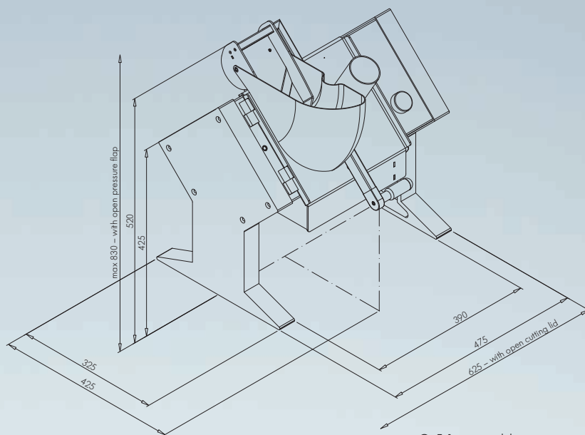
G 5.1 vegetable cutter (Representation)
